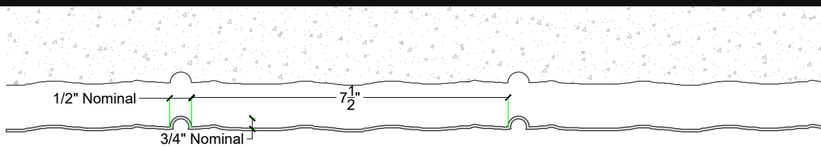
ELEVATION VIEW
